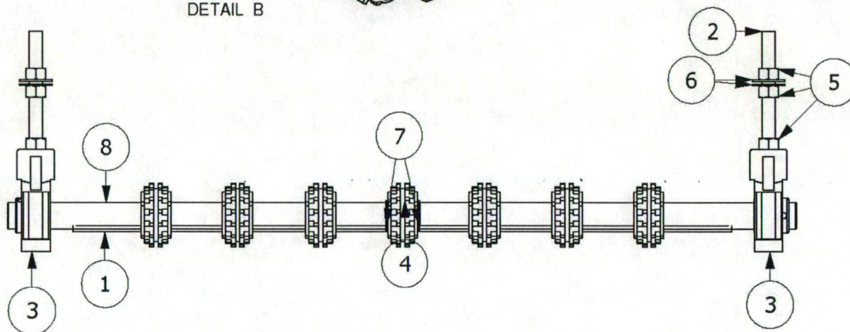
DETAIL B
